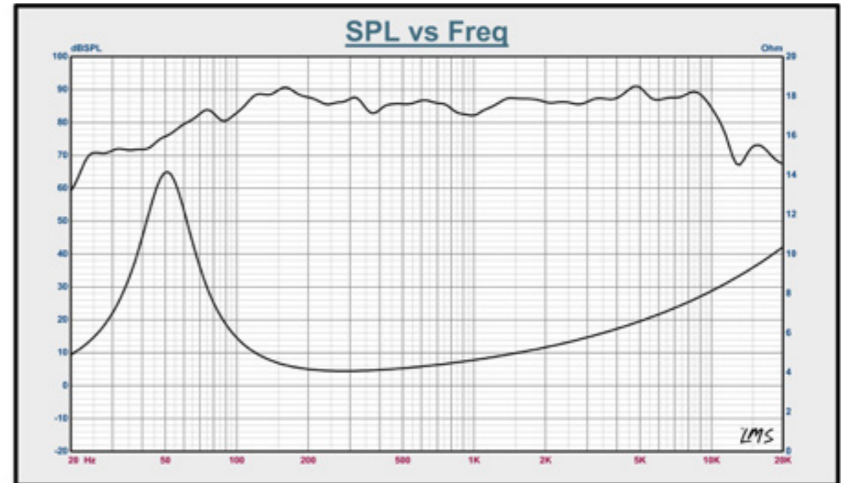
Legatia L6SE Frequency Response Graph
