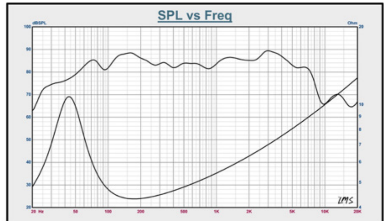
Legatia L8SE Frequency Response Graph
