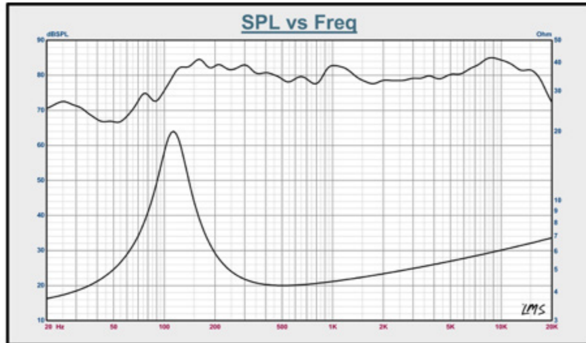
Legatia L3SE Frequency Response Graph
