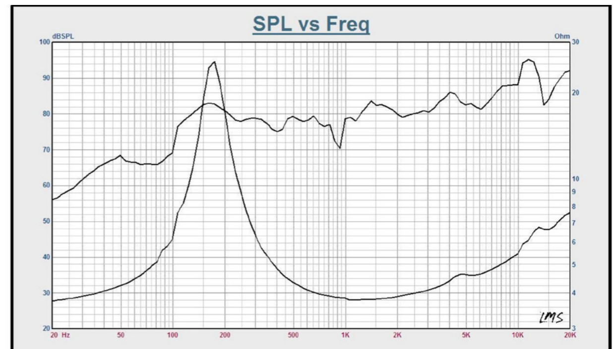
Legatia L2SE Frequency Response Graph
